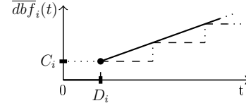
Figure 1: Approximate demand bound function of a sporadic task
