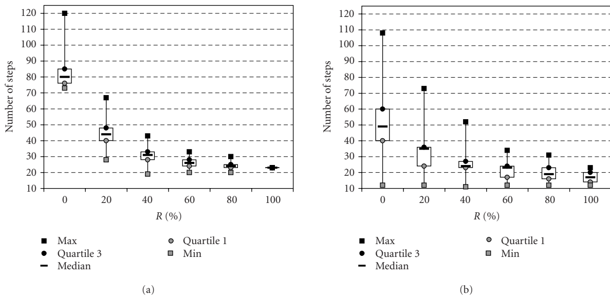
FIGURE 12: Box-and-whisker plots for the random crash test with multiple redundancy configuration settings with n = 12 .
