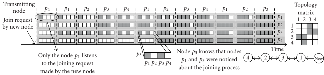
FIGURE 6: Example of the agreement vector update.
