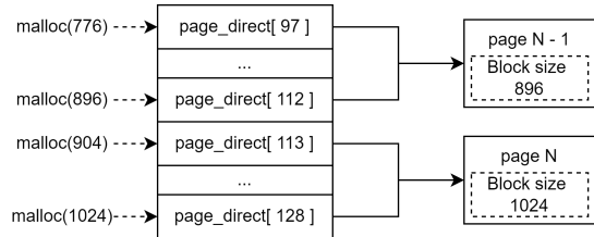
Fig. 6: Some entries of the pages_direct array that point to the same page.
