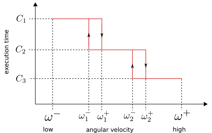
Figure 5: Hysteresis
