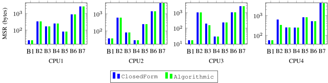
Figure 7. MSR for the STR2RTS benchmark suite when nodes are partitioned according to the worst-fit WCET partitioning scheme on a multiprocessor platform composed of M = 4 processors.
