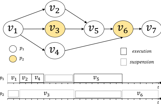
Figure 2. Example scheduling of a DAG task partitioned onto two processors. Nodes v_1, v_2, v_4, v_5 , and v_7 are allocated to p_1 , while nodes v_3 and v_6 are allocated to p_2 . Note that the task is self-suspended on a processor p_k whenever, due to uncompleted predecessors on remote processors, there are no nodes allocated to p_k that are ready for being executed.
