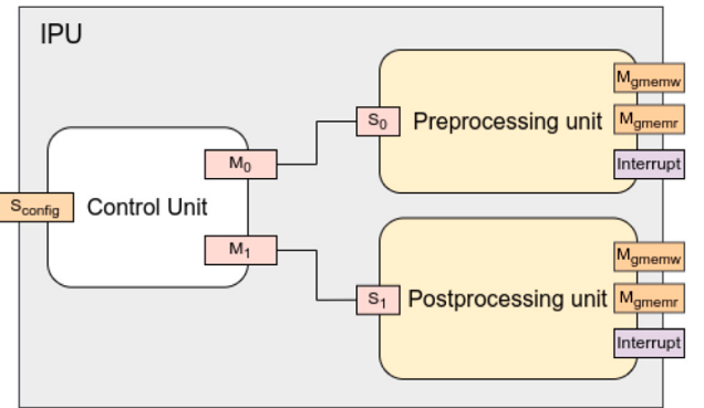
Fig. 5. Architecture of the image processing unit.
