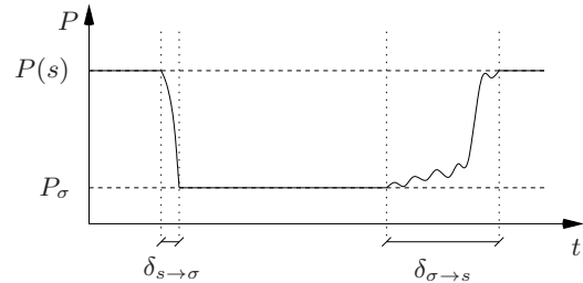
Fig. 3. Overhead due to switching from active to sleep state and viceversa.
